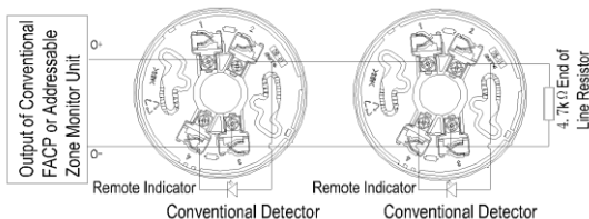
The typical connection of End of Line Resistor
