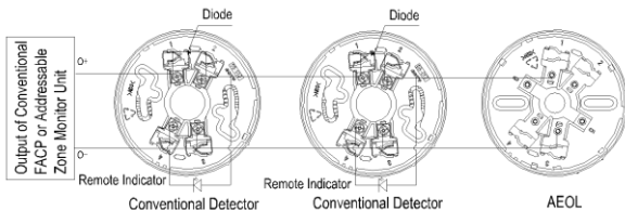
The typical connection of End of Line Resistor
