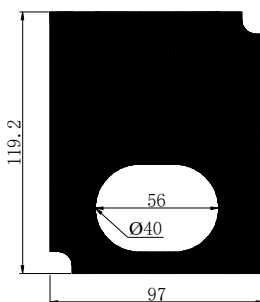
Fig.11c (unit: mm)
